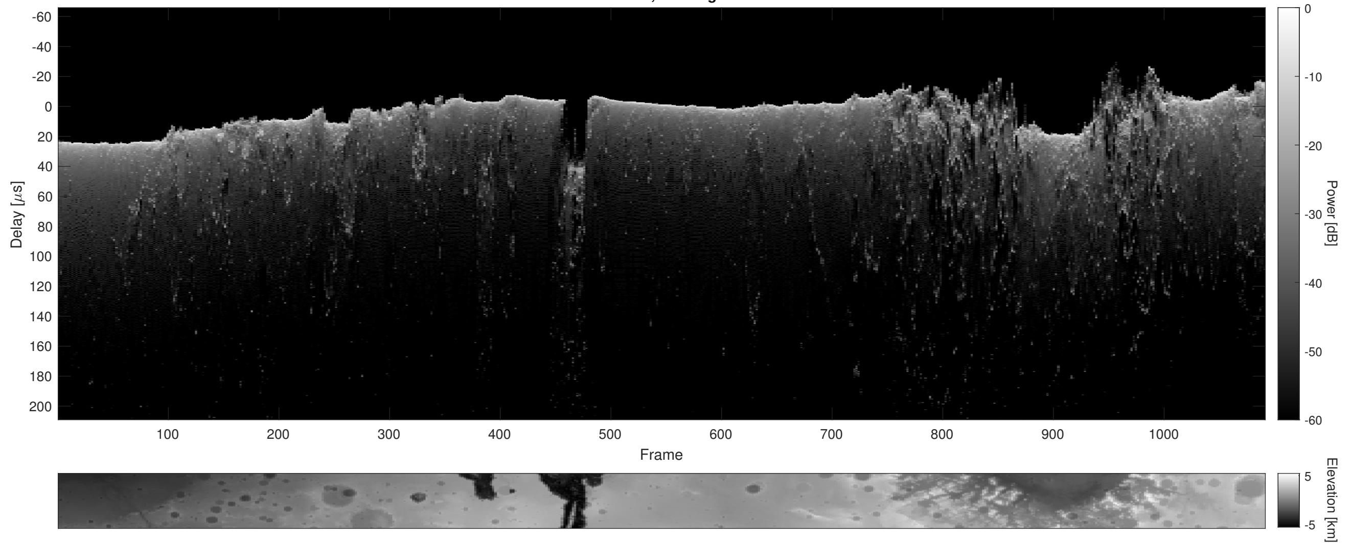
Orbit 5019, Cluttergram
