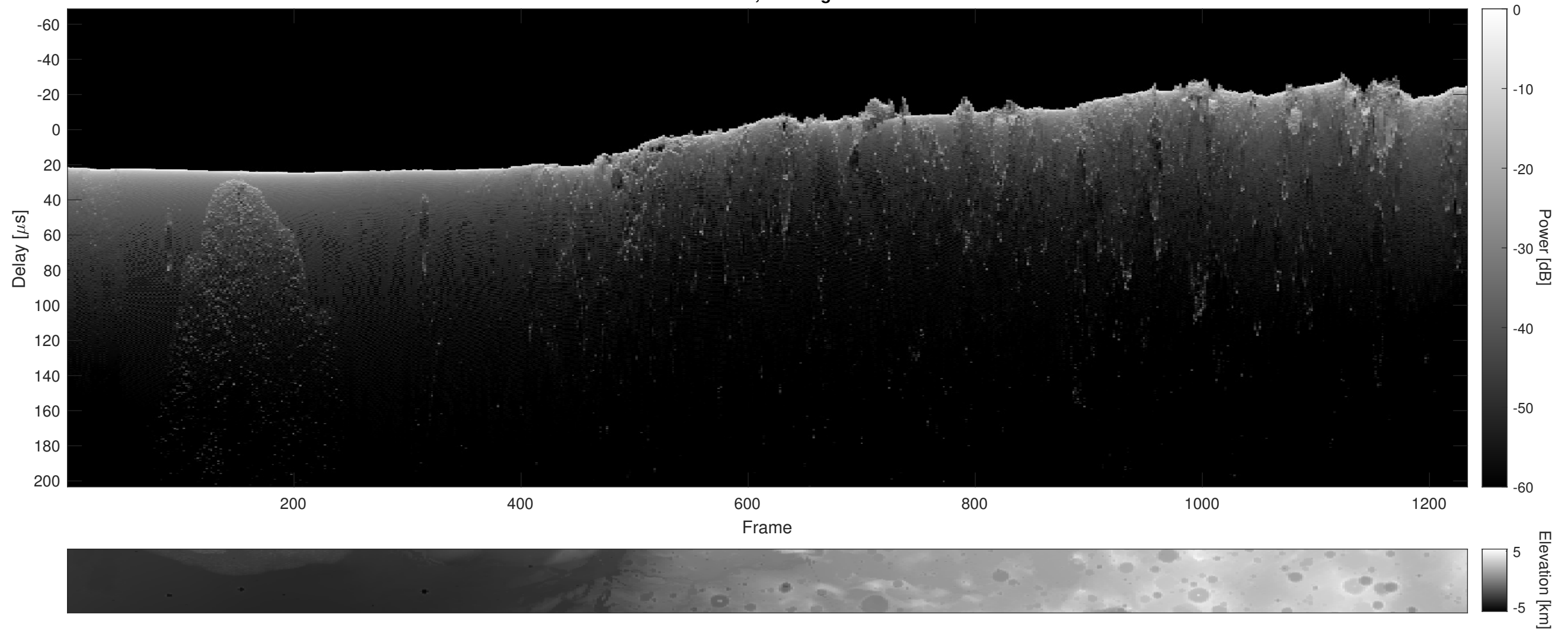
Orbit 5020, Cluttergram
