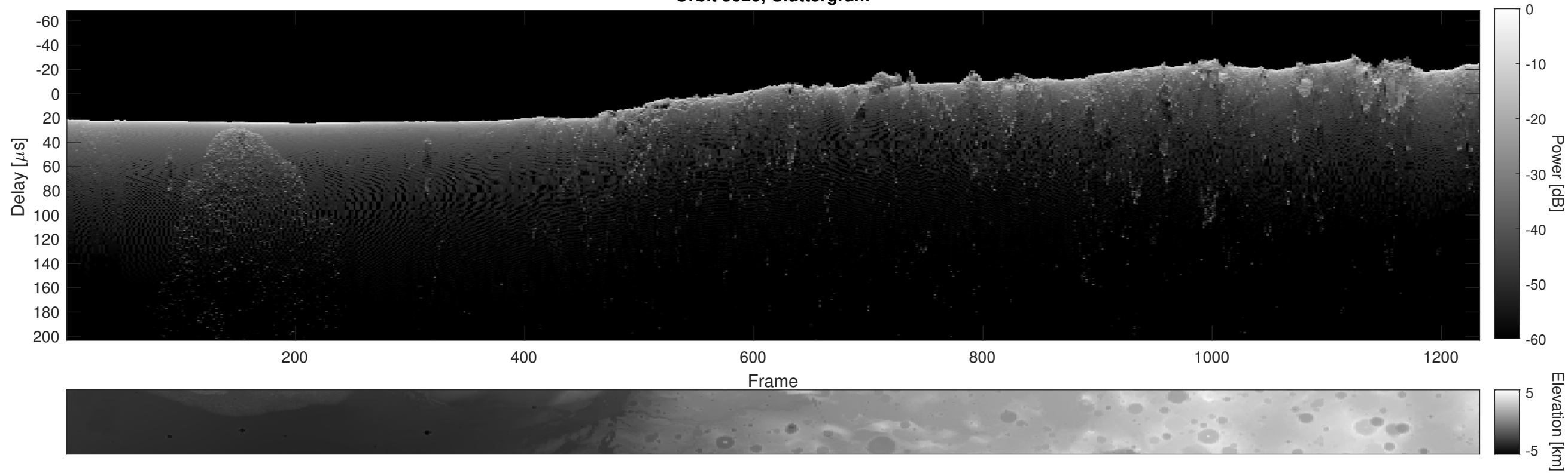
Orbit 5020, Cluttergram
