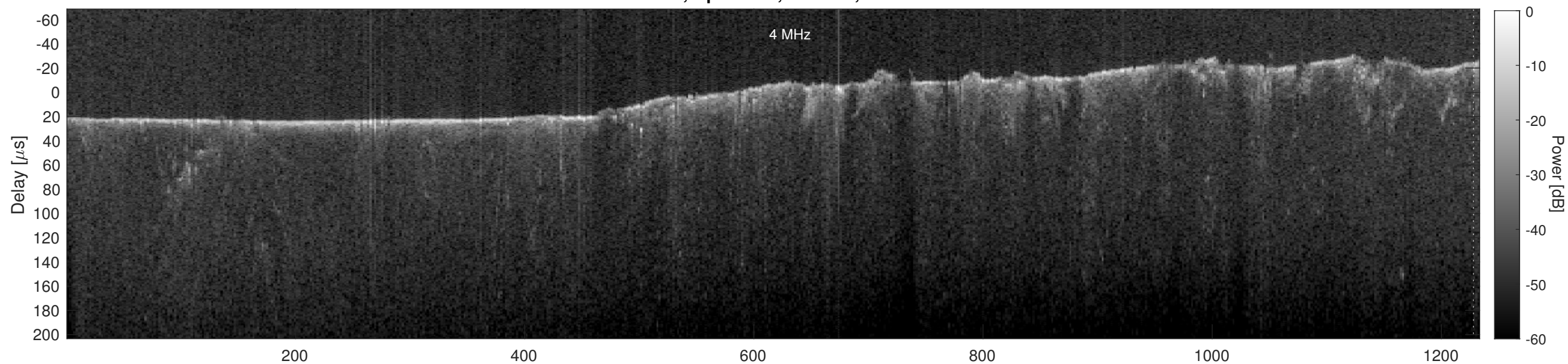
Orbit 5020, Cluttergram
