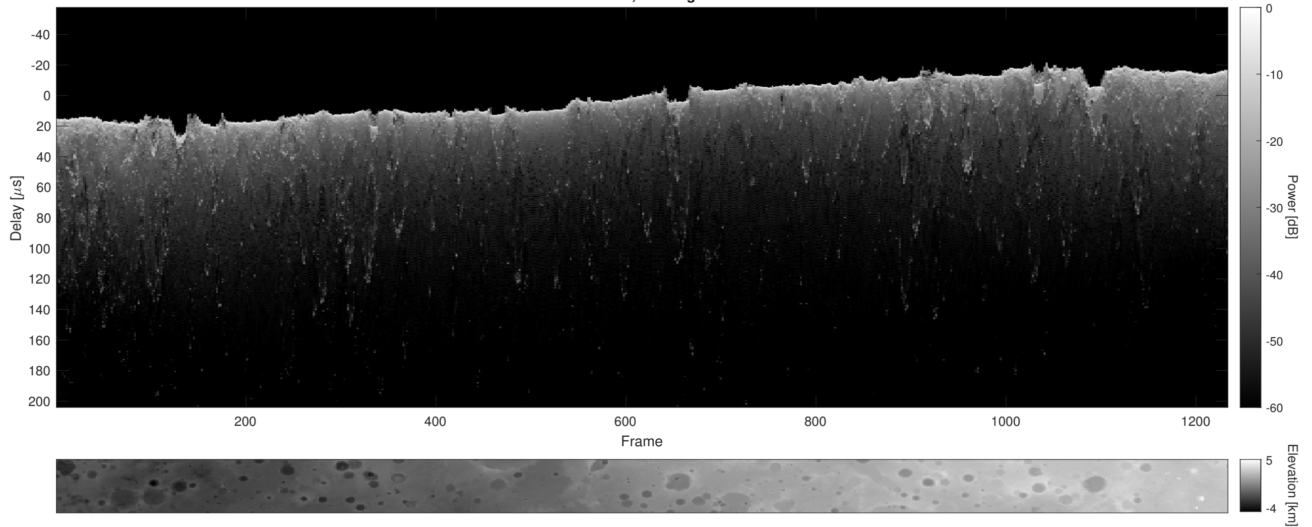
Orbit 5022, Cluttergram
