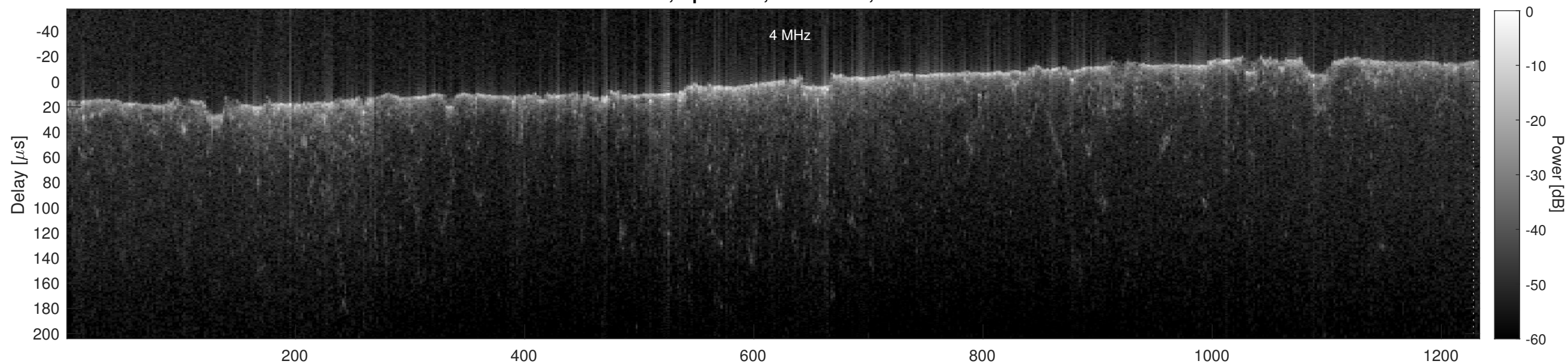
Orbit 5022, Cluttergram
