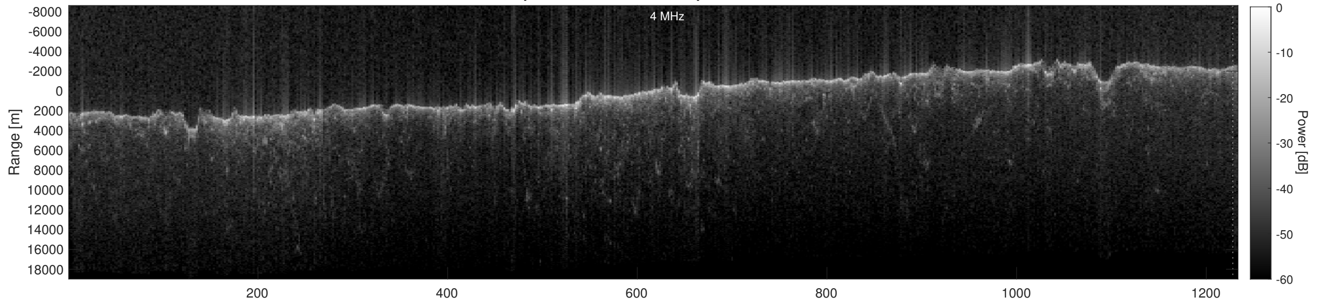
Orbit 5022, Depth-Corrected Cluttergram
