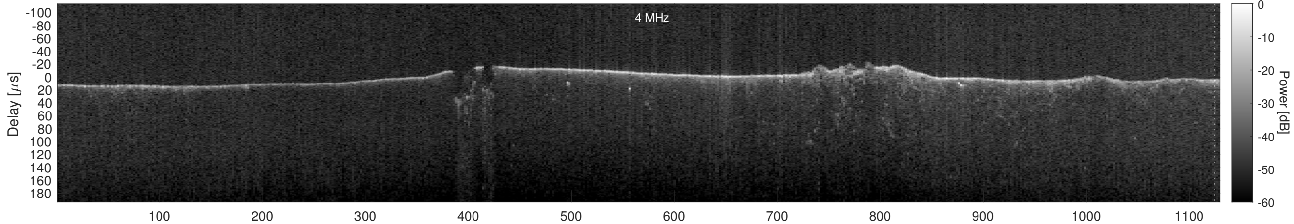
Orbit 5023, Cluttergram
