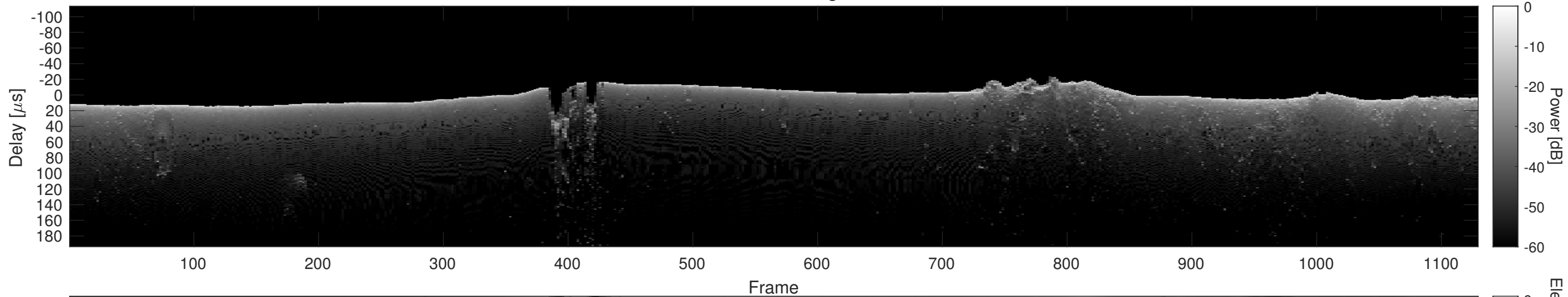
Orbit 5023, Cluttergram
