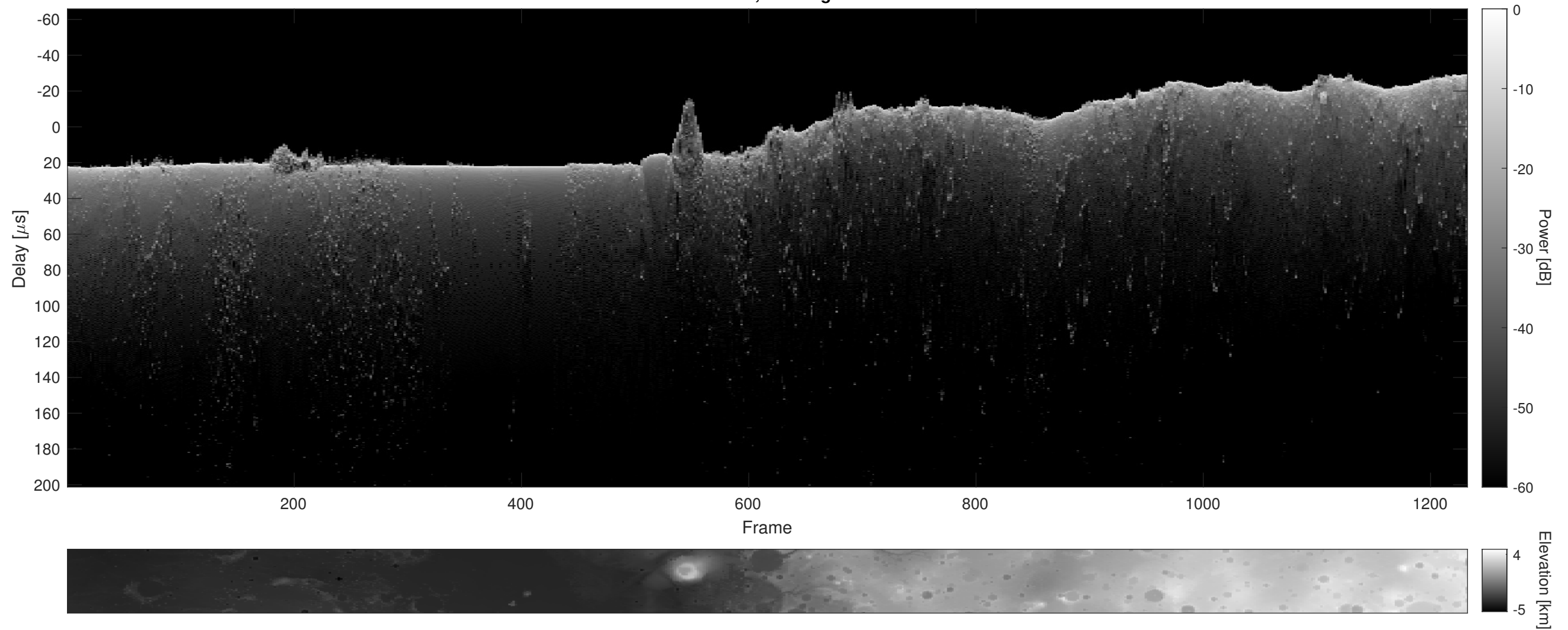
Orbit 5024, Cluttergram
