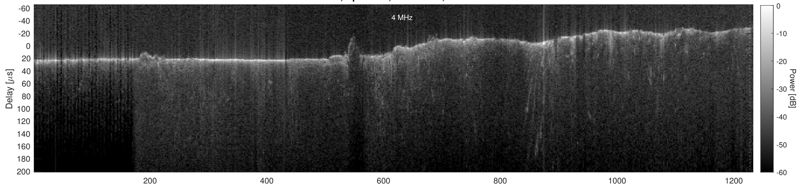
Orbit 5024, Cluttergram
