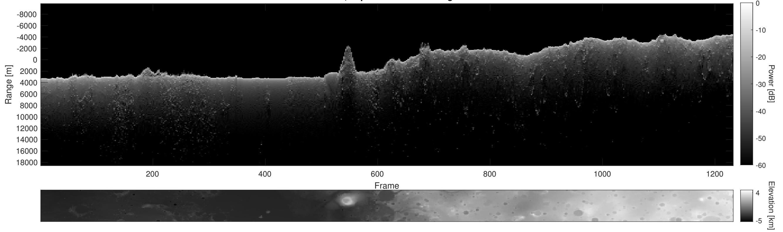
Orbit 5024, Depth-Corrected Cluttergram
