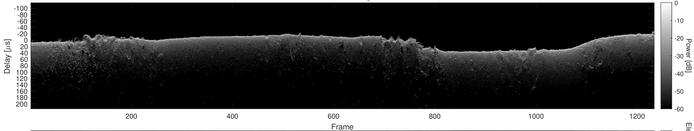
Orbit 5025, Cluttergram
