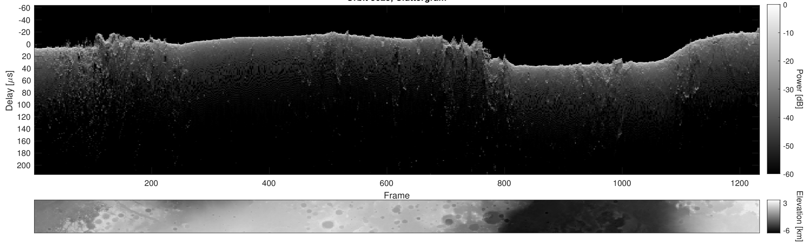
Orbit 5025, Cluttergram
