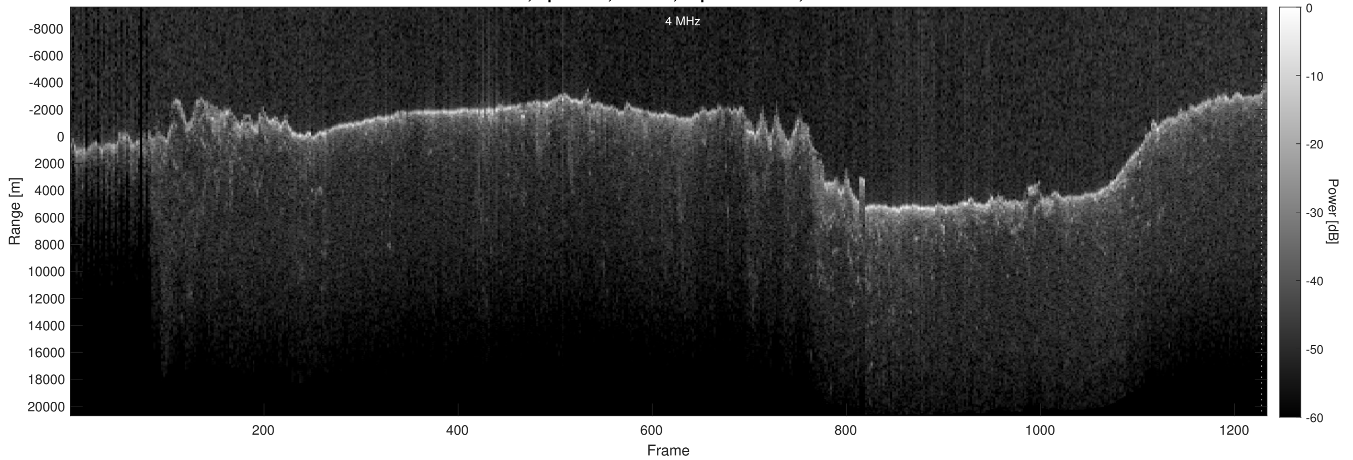
Orbit 5025, Optimized, Window, Depth-Corrected, Channel 2
