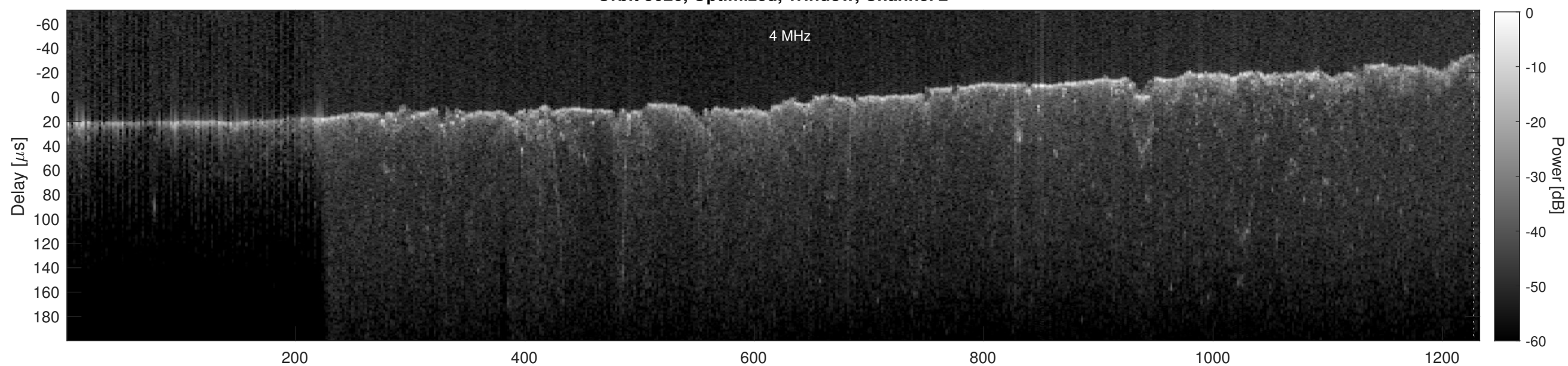
Orbit 5026, Cluttergram
