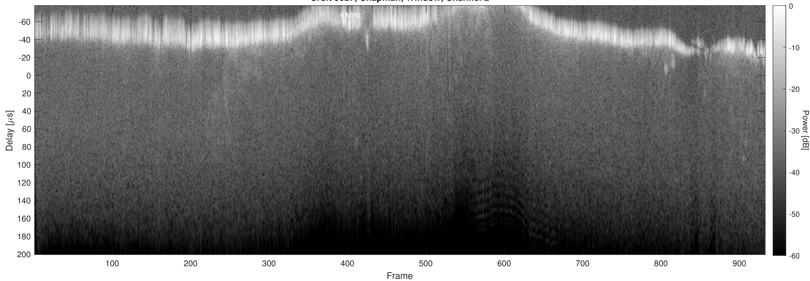
Orbit 5027, Chapman, Window, Channel 2
