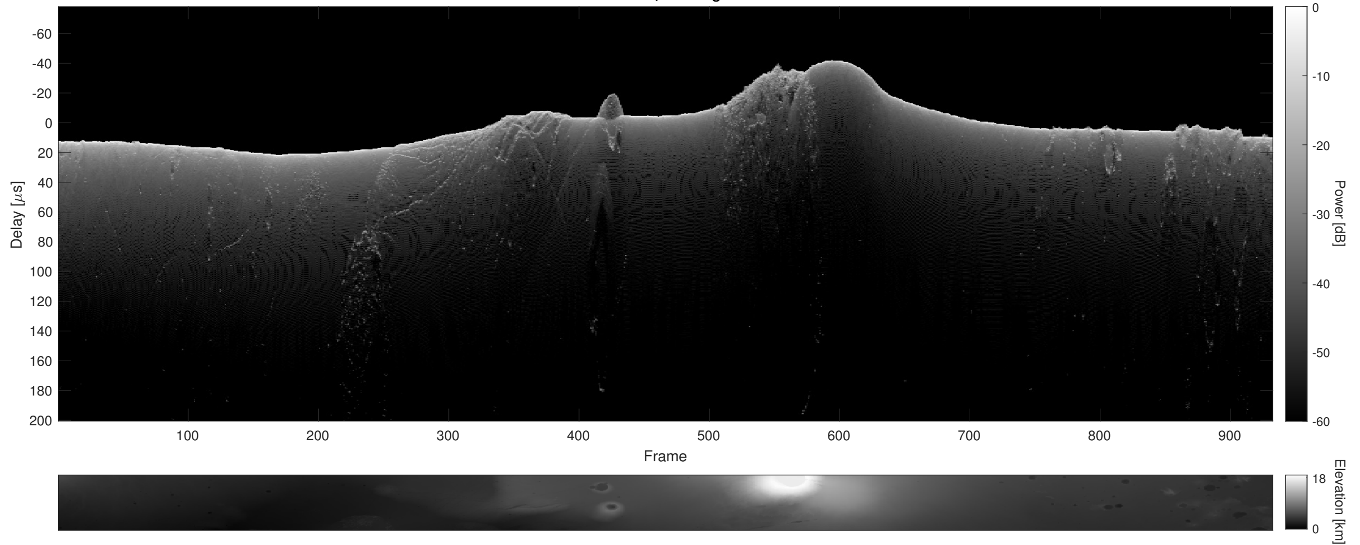
Orbit 5027, Cluttergram
