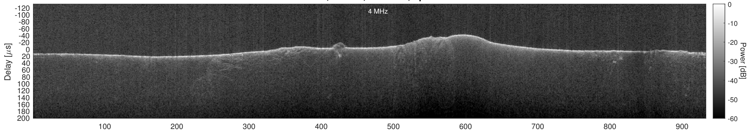
Orbit 5027, Cluttergram
