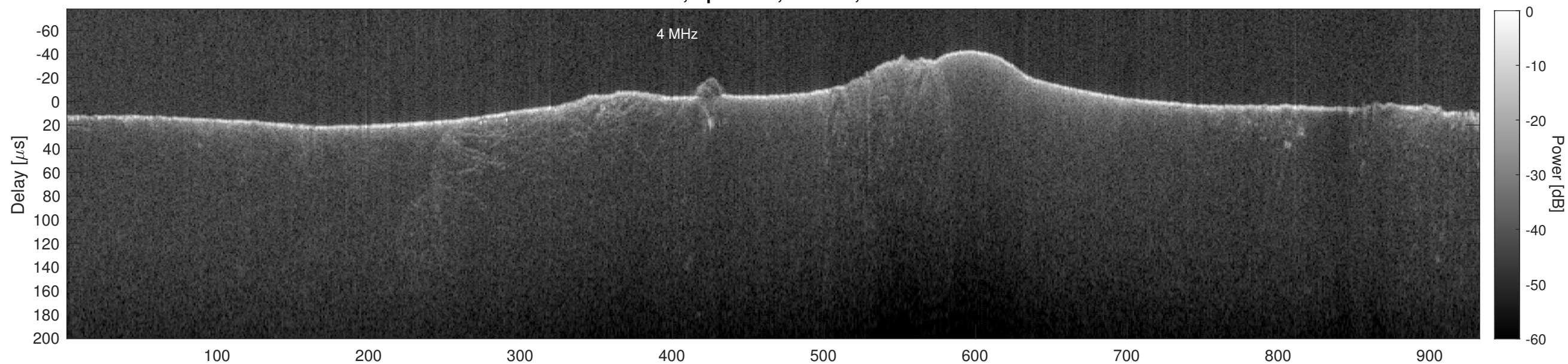
Orbit 5027, Cluttergram
