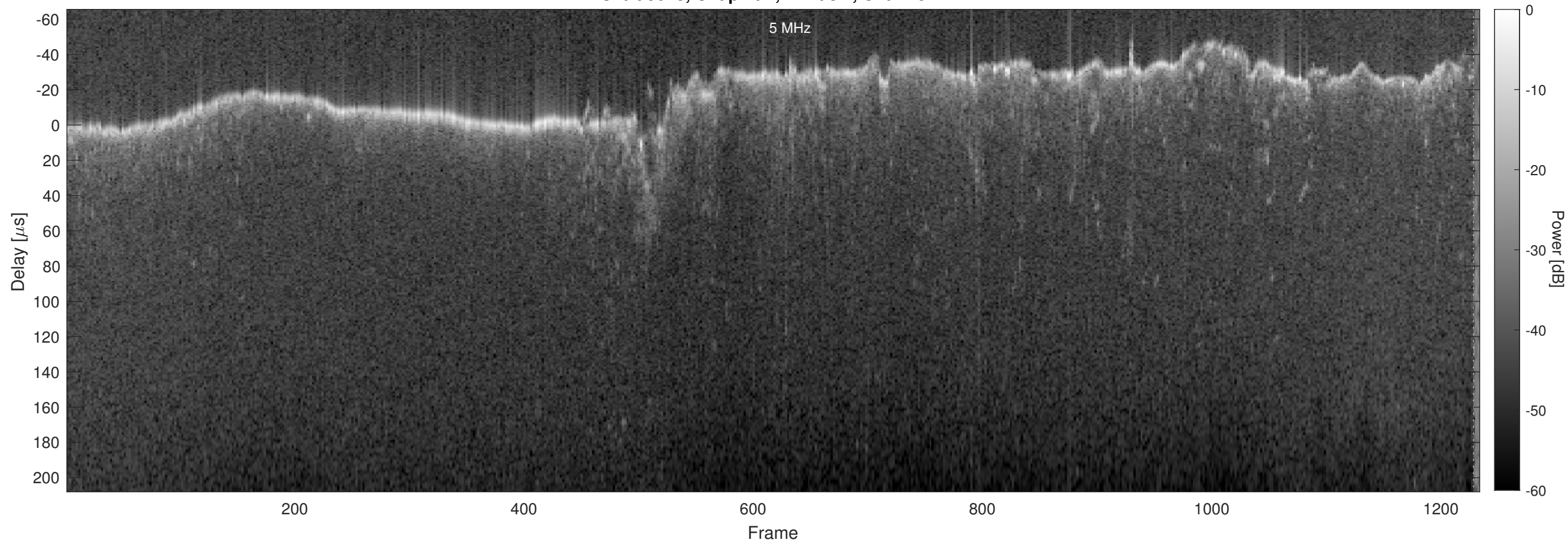
Orbit 5028, Chapman, Window, Channel 2
