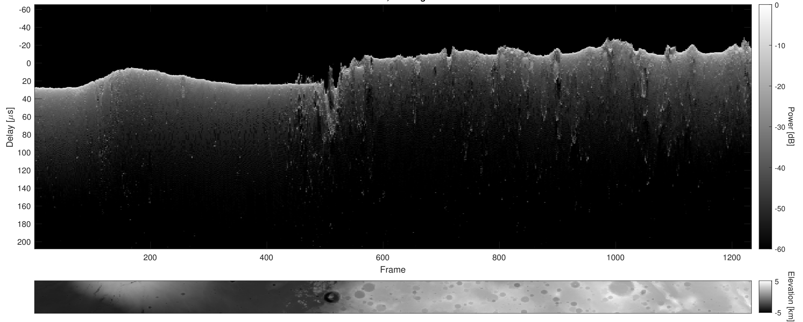
Orbit 5028, Cluttergram
