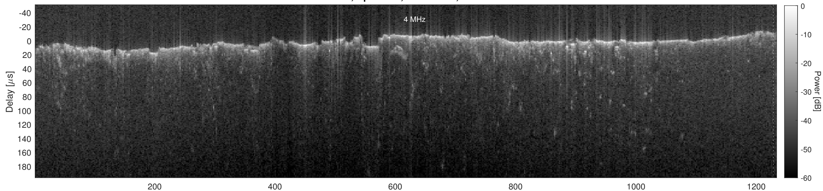
Orbit 5029, Cluttergram
