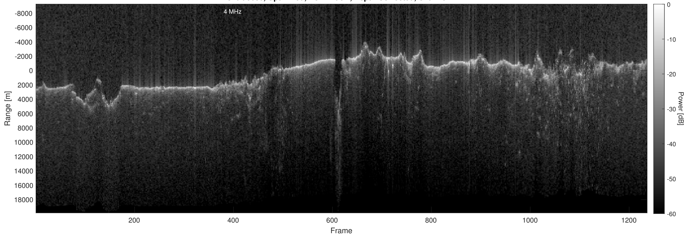
Orbit 5030, Optimized, No Window, Depth-Corrected, Channel 2
