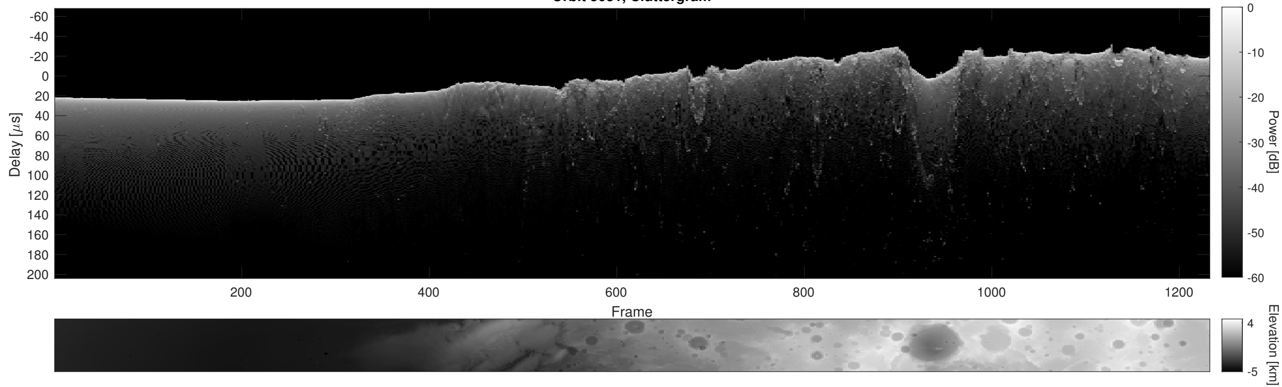
Orbit 5031, Cluttergram
