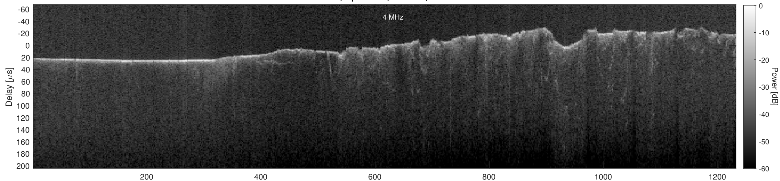
Orbit 5031, Cluttergram
