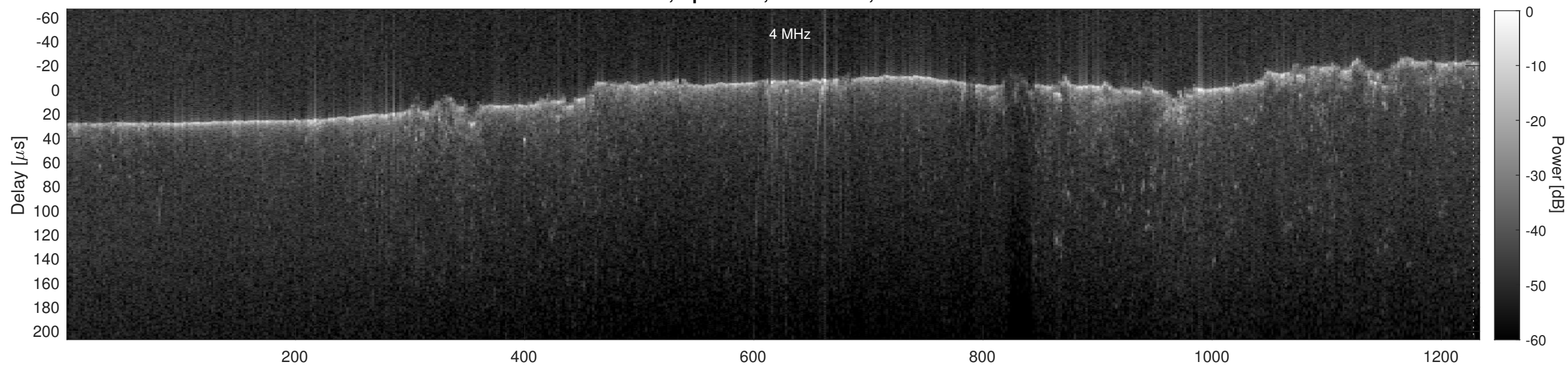
Orbit 5032, Cluttergram
