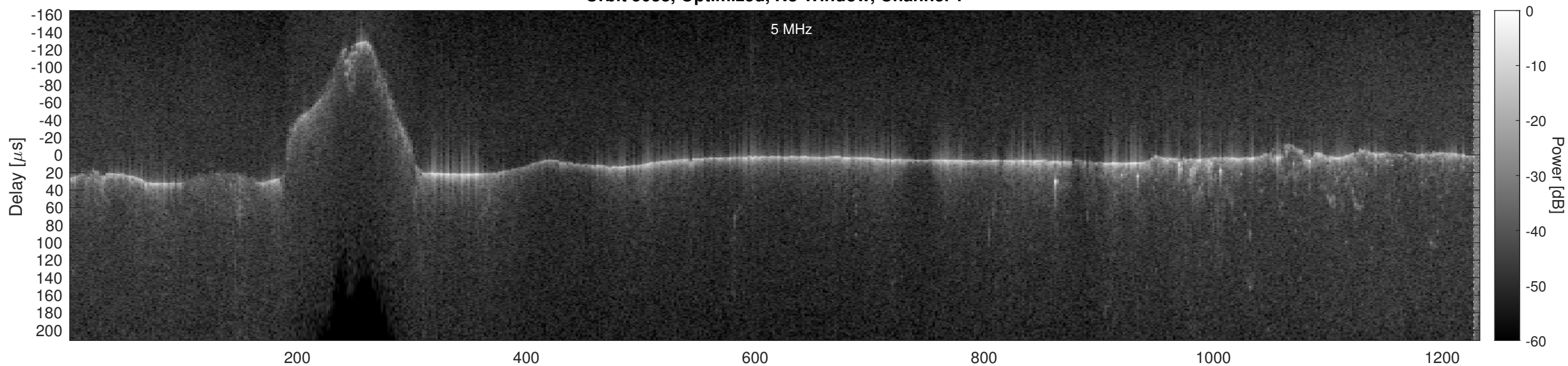
Orbit 5038, Optimized, No Window, Channel 2
