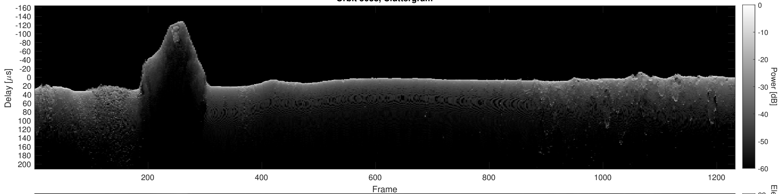
Orbit 5038, Cluttergram
