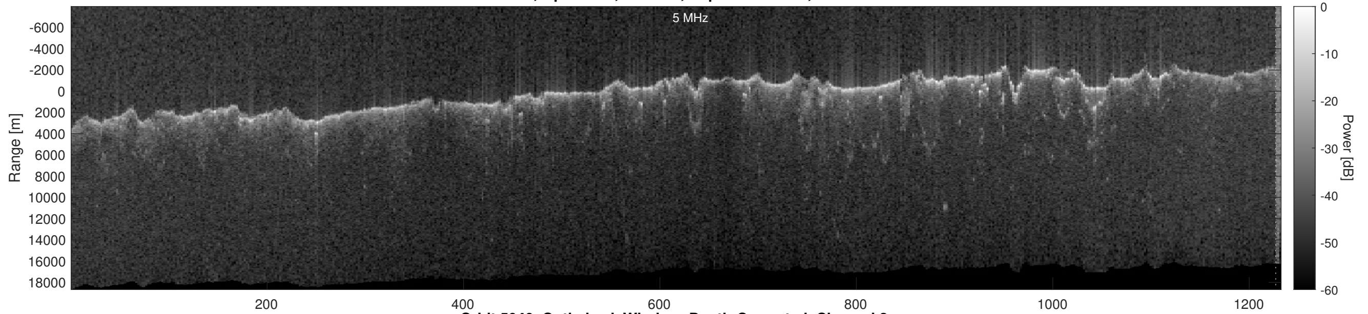
Orbit 5040, Optimized, Window, Depth-Corrected, Channel 2
