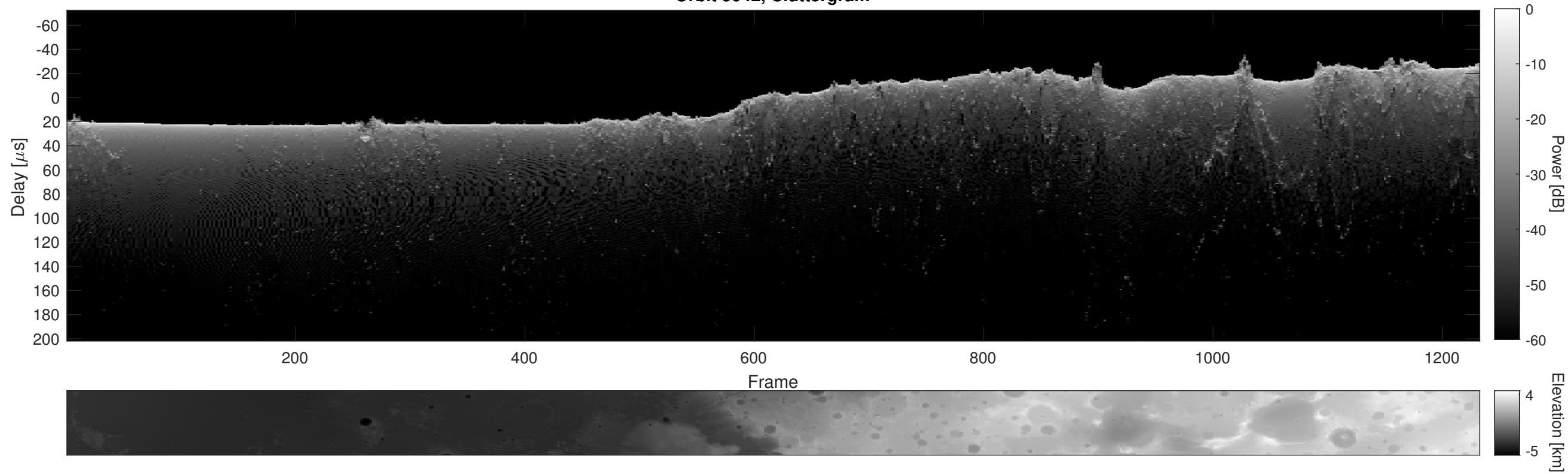
Orbit 5042, Cluttergram
