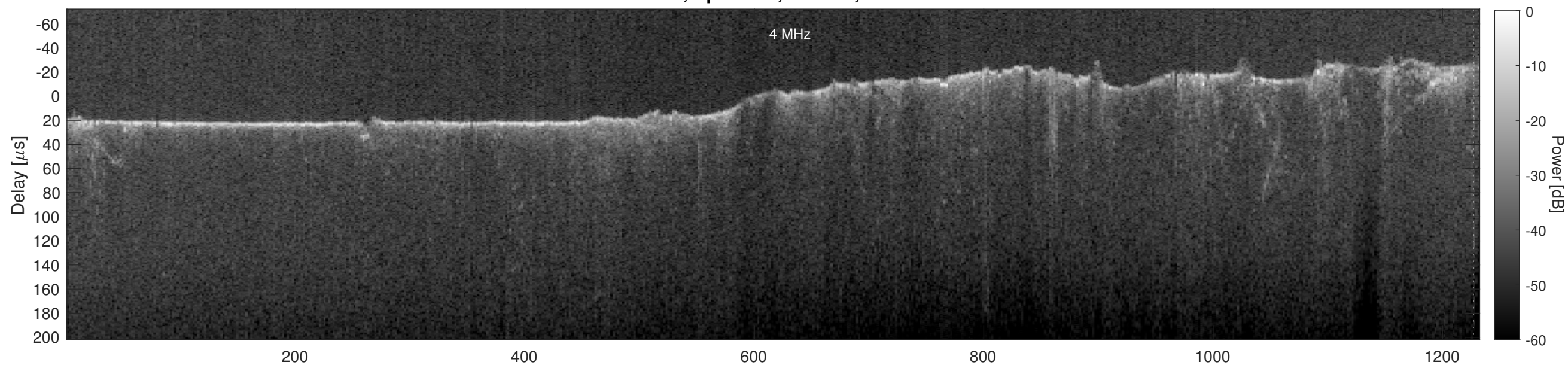
Orbit 5042, Cluttergram
