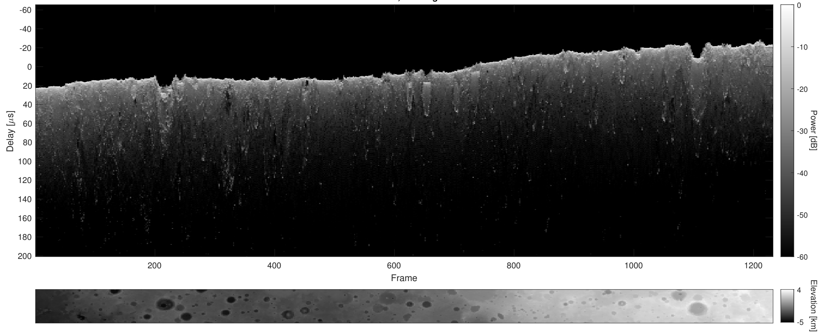
Orbit 5044, Cluttergram
