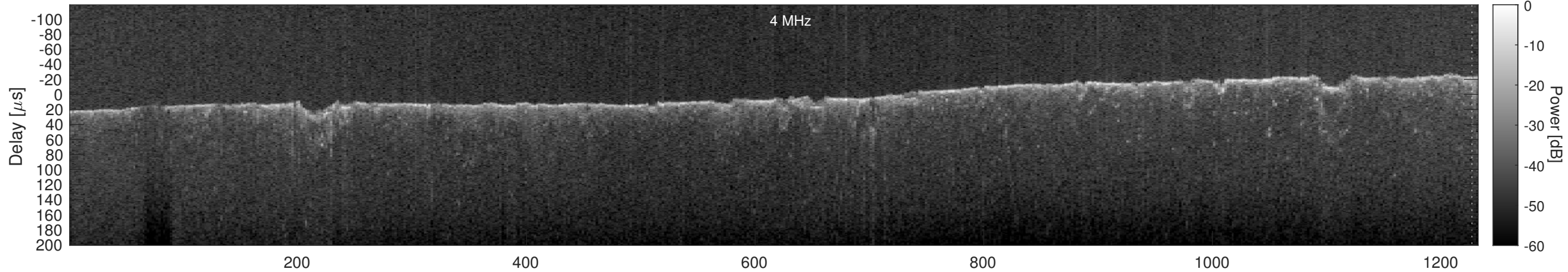
Orbit 5044, Cluttergram
