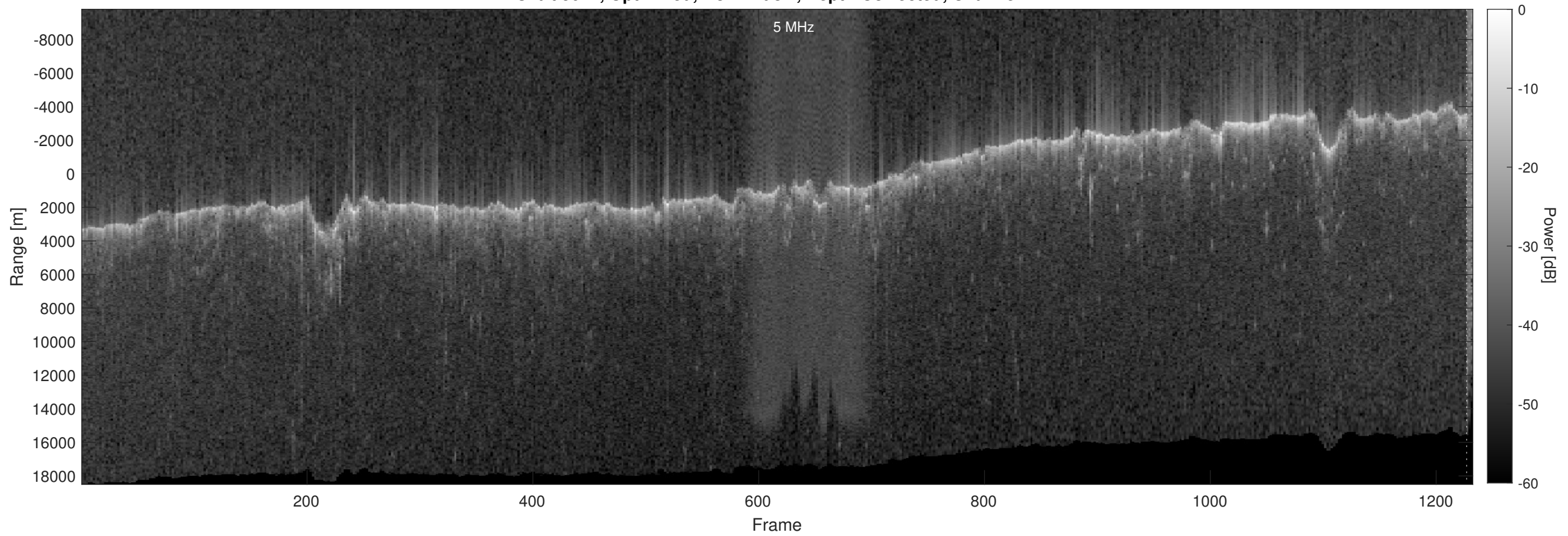
Orbit 5044, Optimized, No Window, Depth-Corrected, Channel 2
