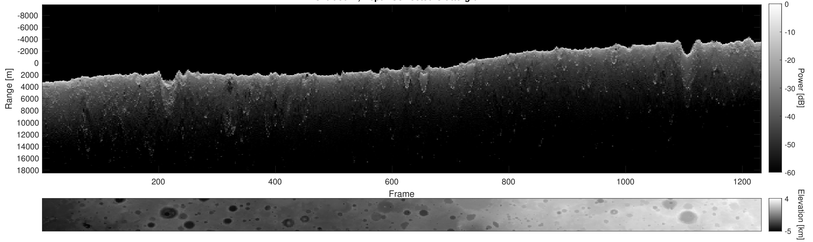
Orbit 5044, Depth-Corrected Cluttergram
