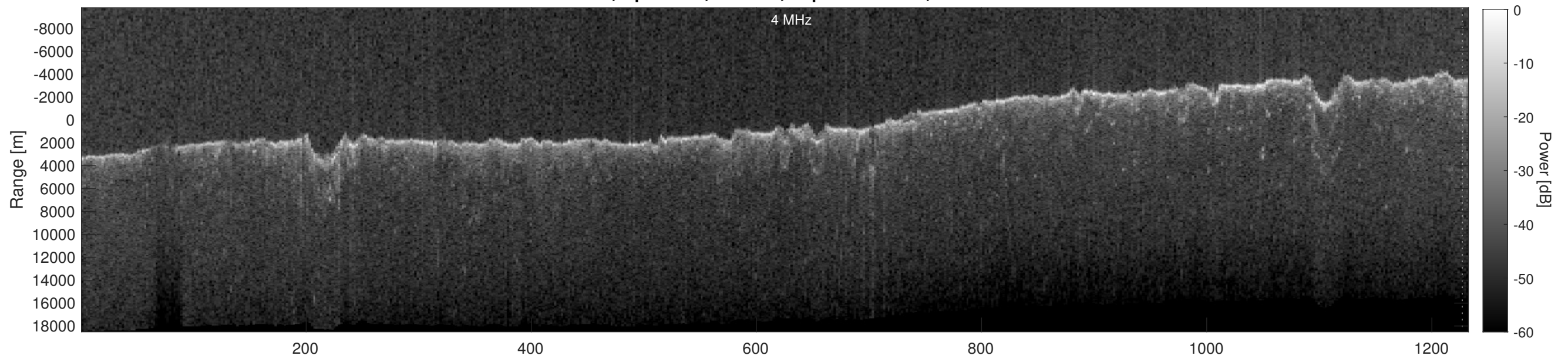
Orbit 5044, Depth-Corrected Cluttergram
