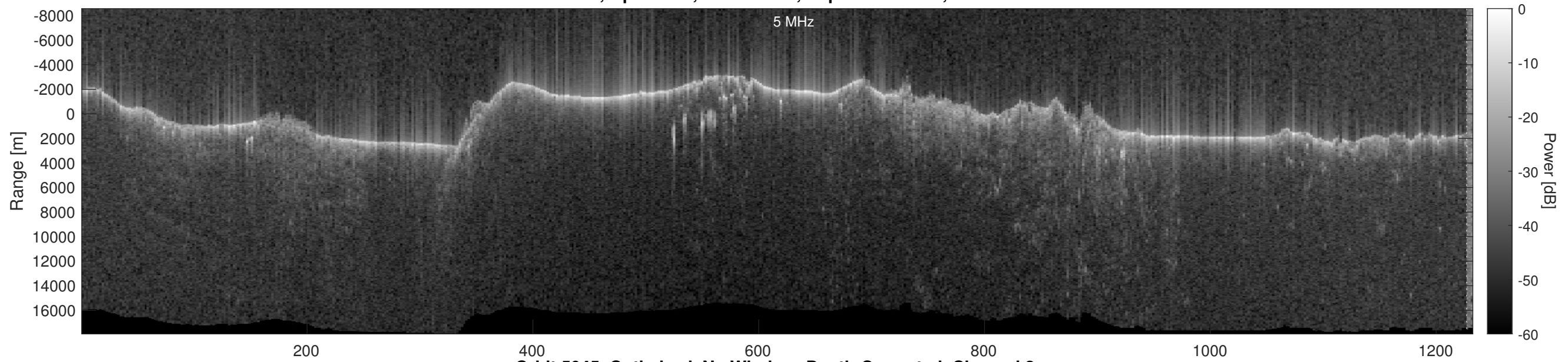
Orbit 5045, Optimized, No Window, Depth-Corrected, Channel 2
