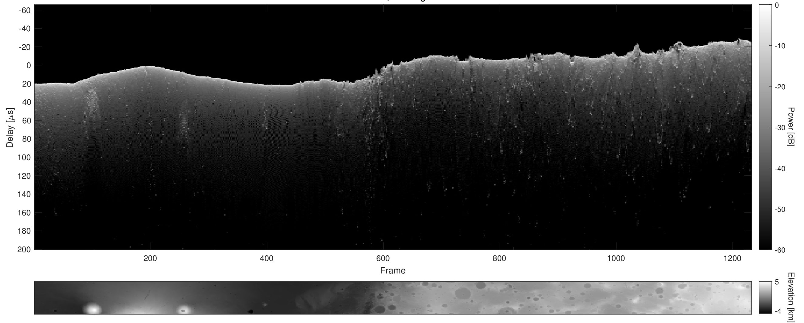
Orbit 5046, Cluttergram
