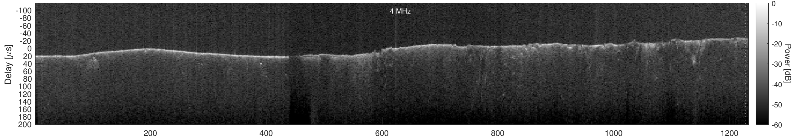
Orbit 5046, Cluttergram
