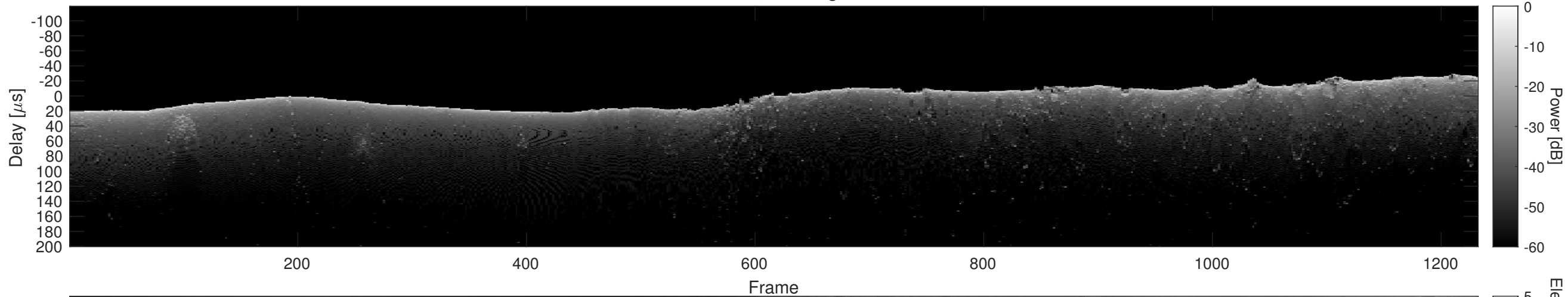
Orbit 5046, Cluttergram
