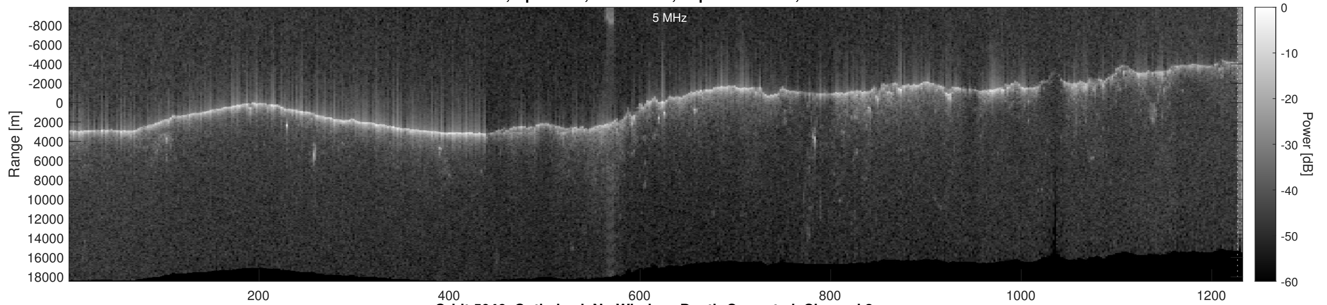
Orbit 5046, Optimized, No Window, Depth-Corrected, Channel 2
