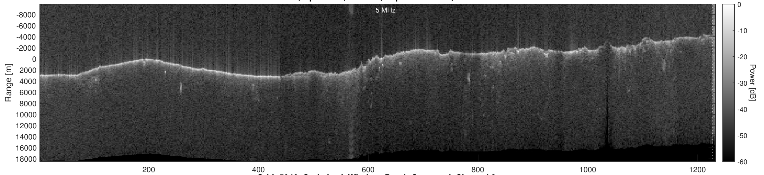
Orbit 5046, Optimized, Window, Depth-Corrected, Channel 2
