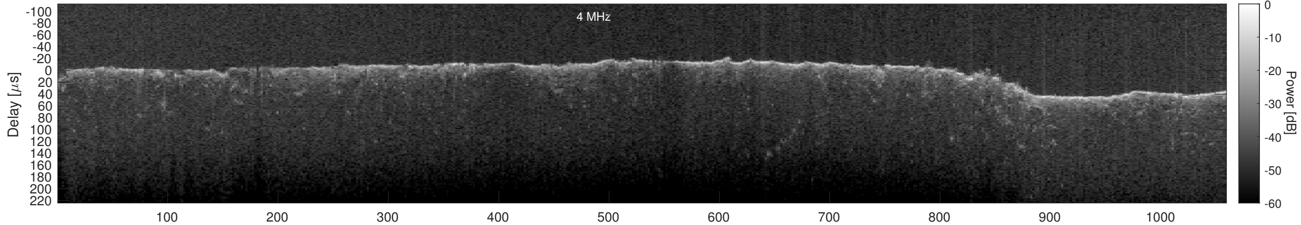
Orbit 5047, Cluttergram
