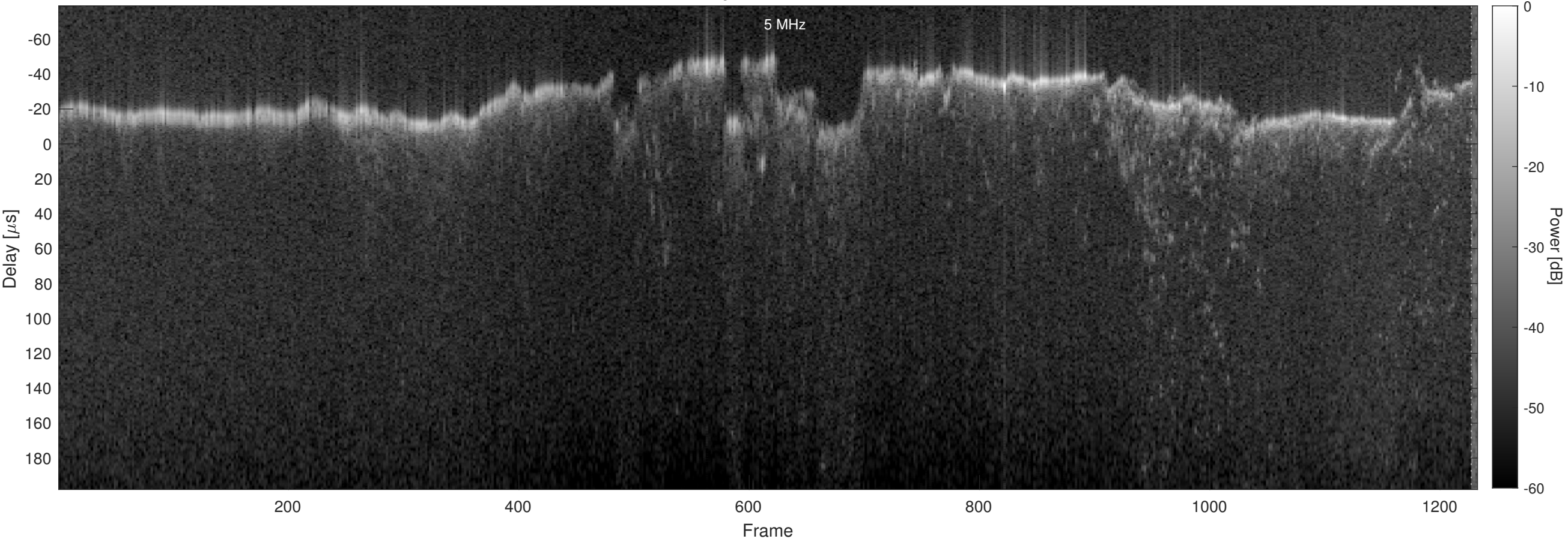
Orbit 5048, Chapman, Window, Channel 2
