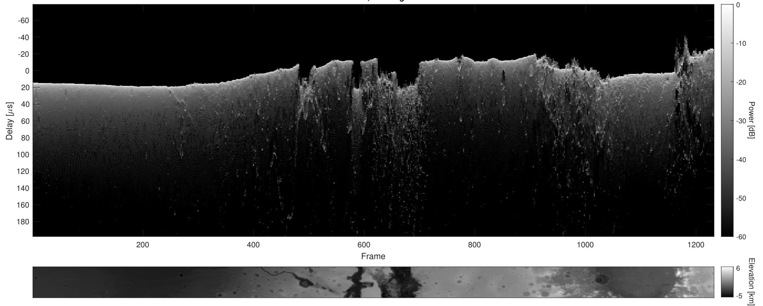
Orbit 5048, Cluttergram
