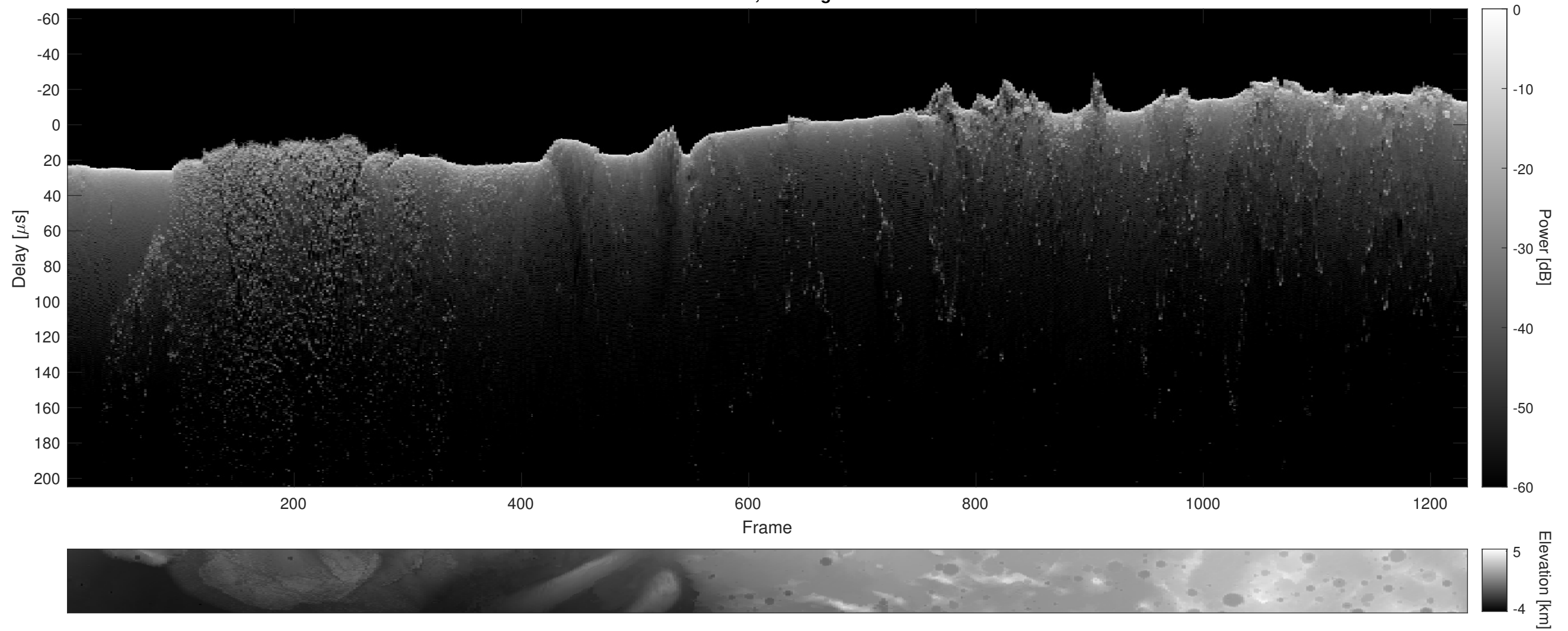
Orbit 5049, Cluttergram
