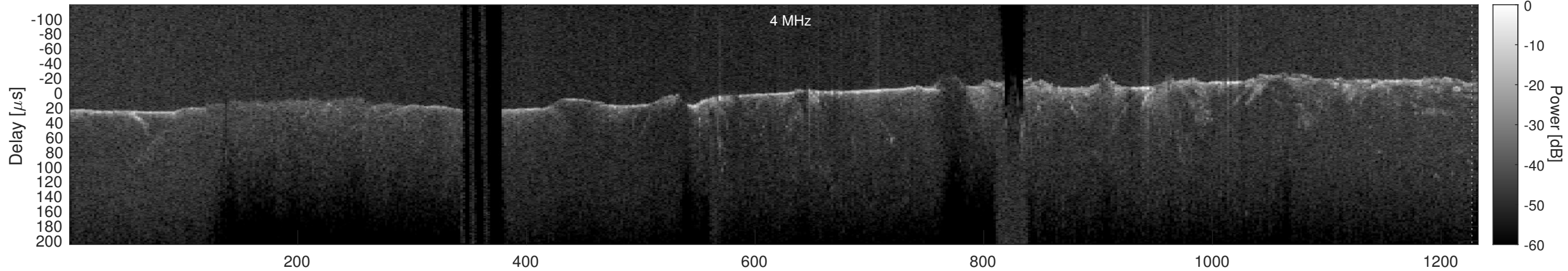
Orbit 5049, Cluttergram
