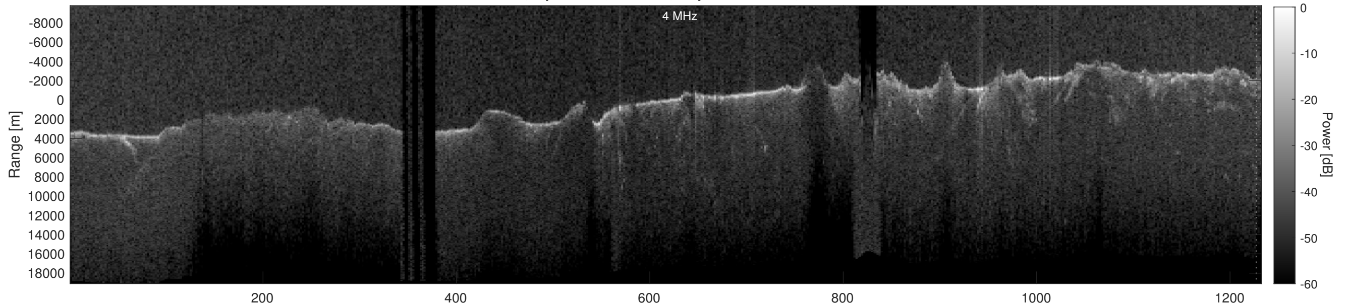
Orbit 5049, Depth-Corrected Cluttergram
