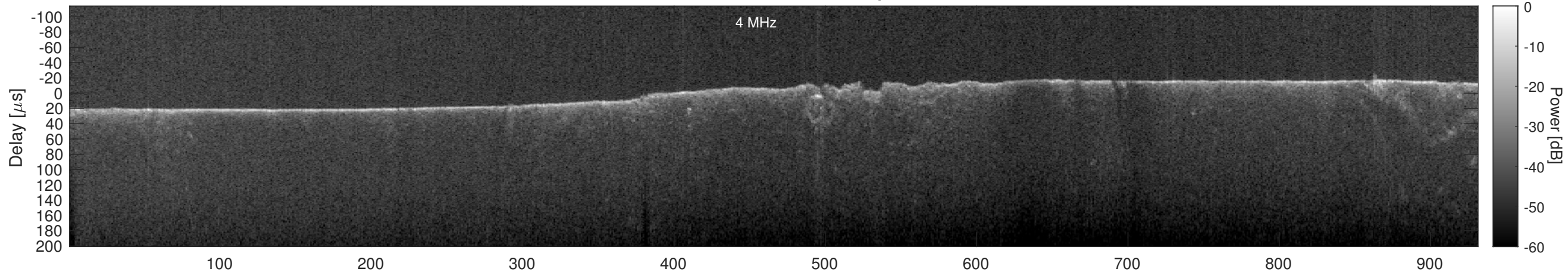
Orbit 5050, Cluttergram
