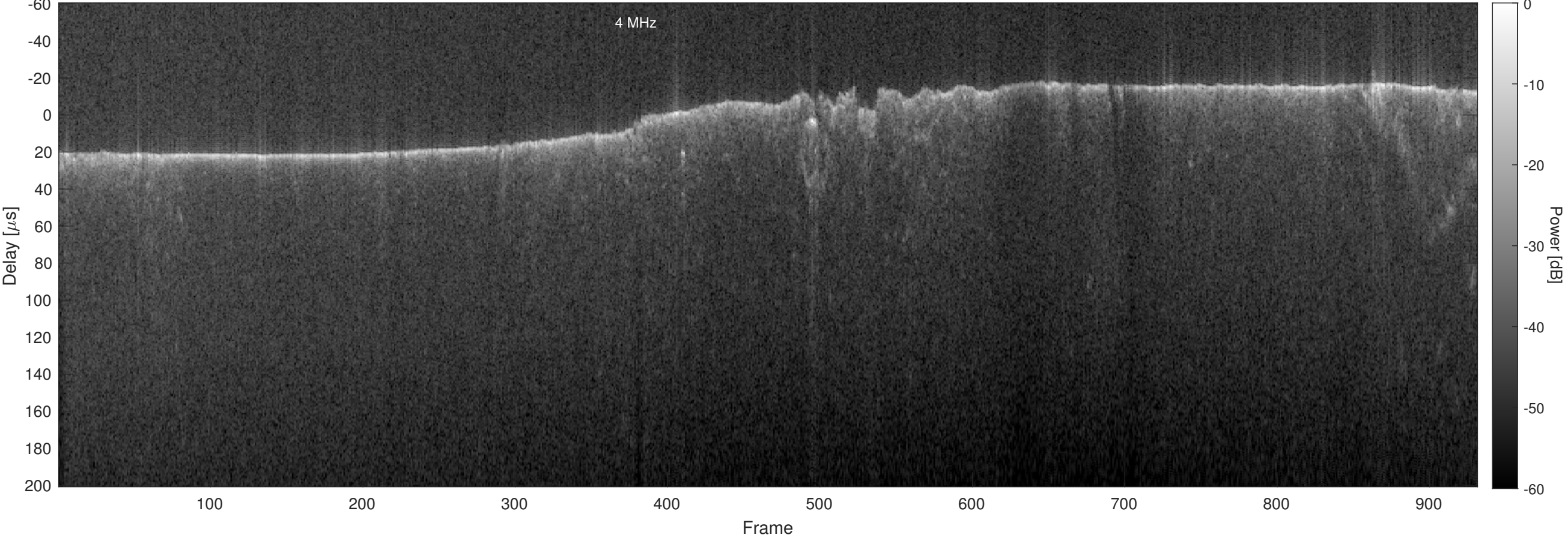
Orbit 5050, Optimized, No Window, Channel 2
