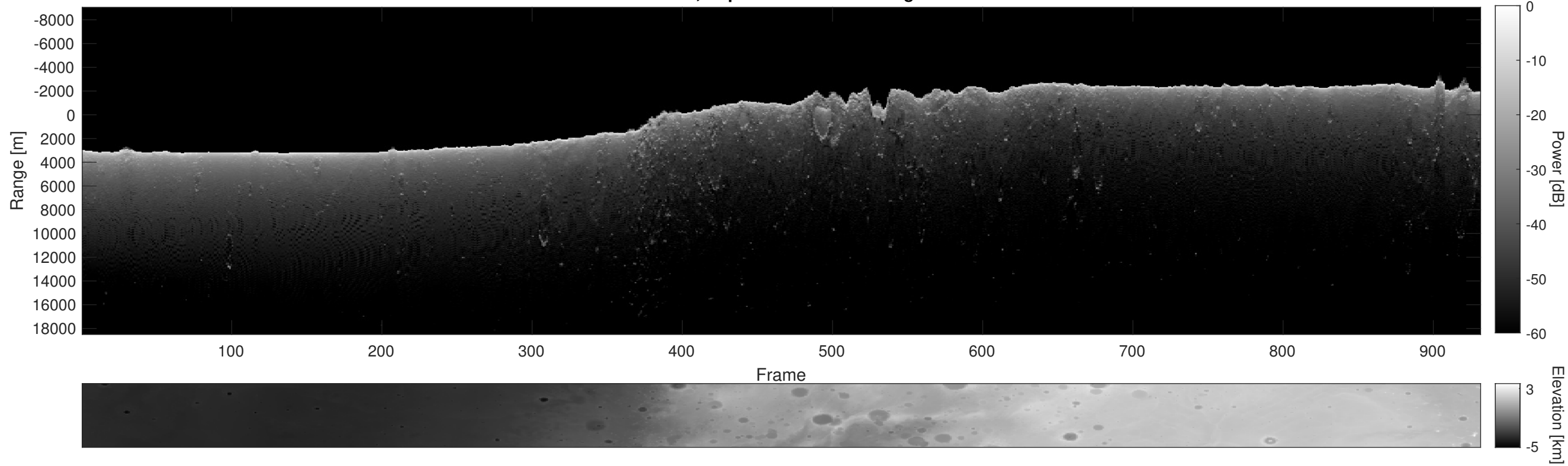
Orbit 5050, Depth-Corrected Cluttergram
