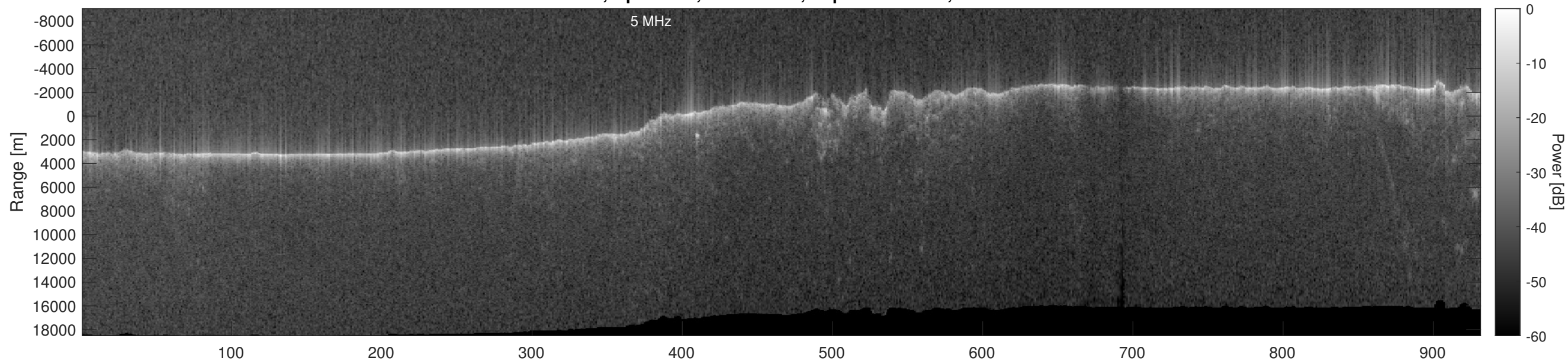
Orbit 5050, Optimized, No Window, Depth-Corrected, Channel 2
