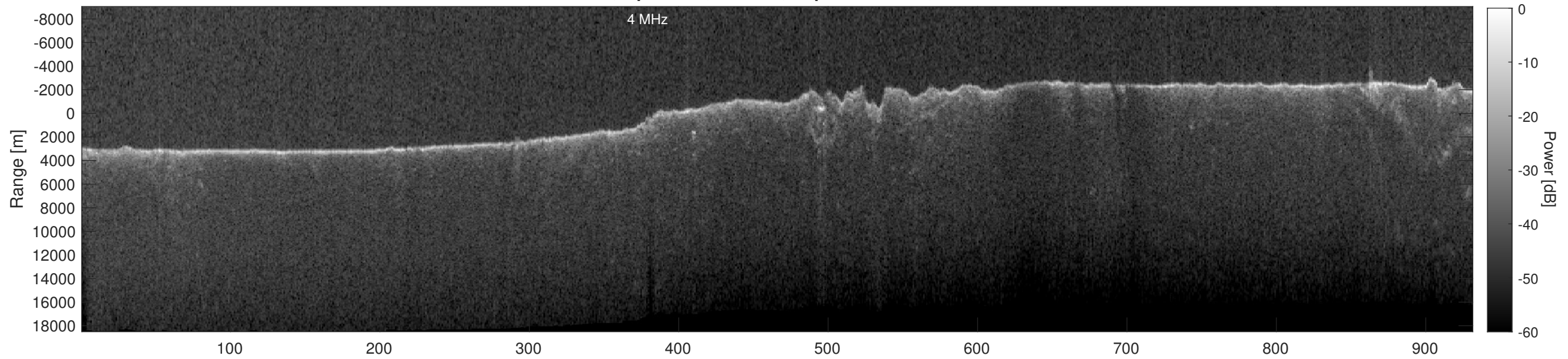
Orbit 5050, Depth-Corrected Cluttergram
