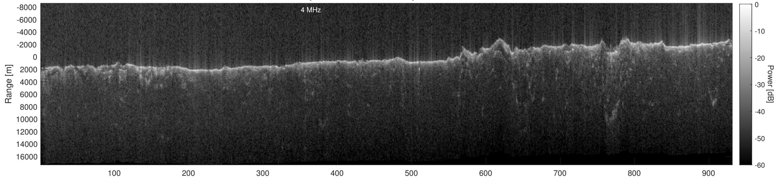
Orbit 5051, Depth-Corrected Cluttergram
